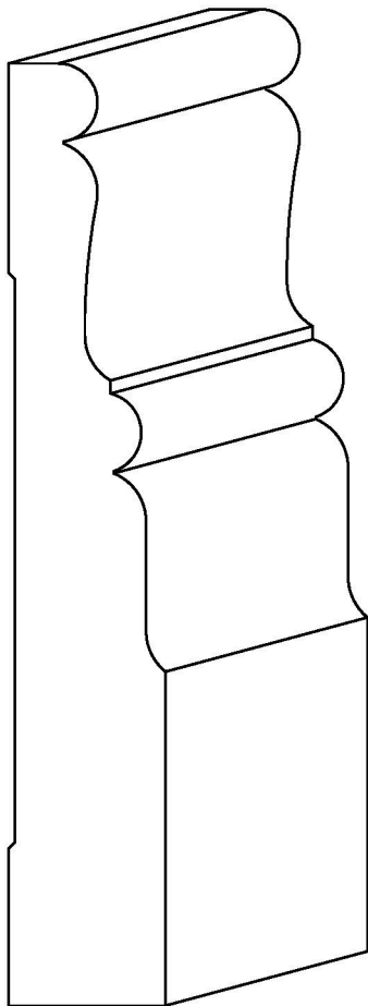
PT 730 Base 1 1/16" x 4-1/2"
