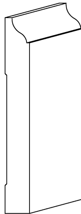
PT 520 Base 7/16" x 3-1/2"
