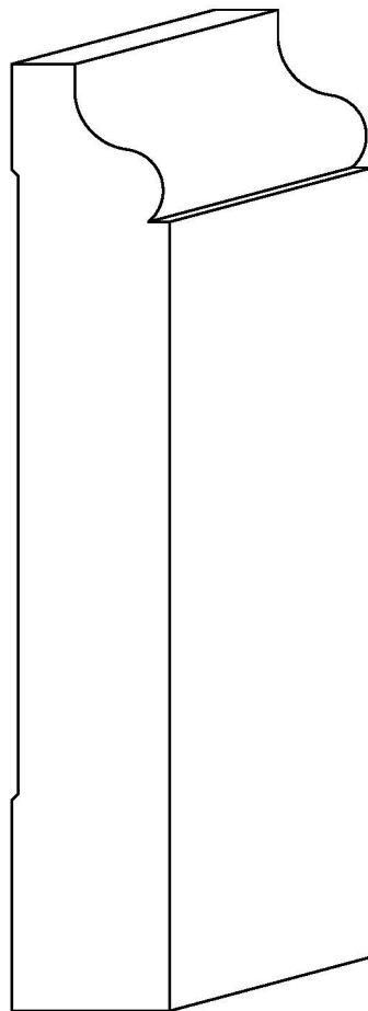
PT 620C Base 3/4" x 4-1/2"
