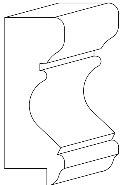
PT 437R Chair Rail 1-1/16" x 3" with 3/4" Rabbet
