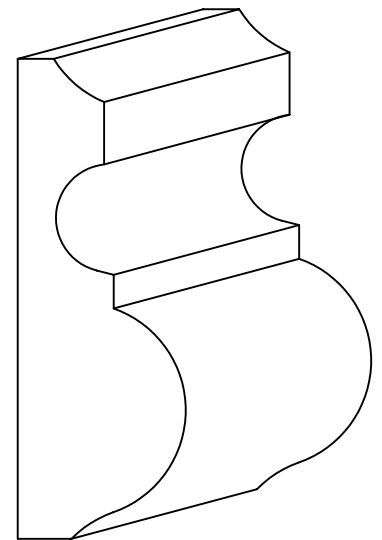
PT 299 NR Chair Rail 7/8" x 2-1/2"
