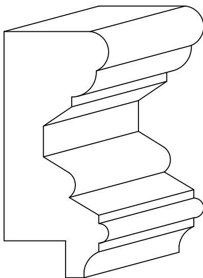
PT 426R Chair Rail 1-1/16" x 2-1/2" 3/8" or 5/8" Rabbet
