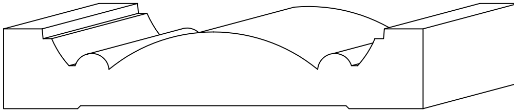
PT 1253 Casing 13/16" x 4-1/4"
