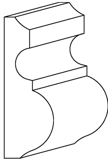
PT 299 NR Chair Rail 7/8" x 2-1/2"
