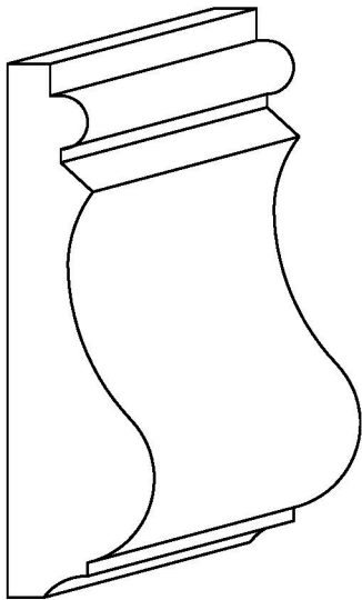
WM 390 Chair Rail 11/16" x 2-1/2"
