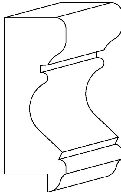
PT 437R Chair Rail 1-1/16" x 3" with 3/4" Rabbet
