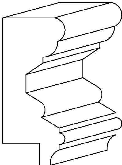
PT 426R Chair Rail 1-1/16" x 2-1/2" 3/8" or 5/8" Rabbet
