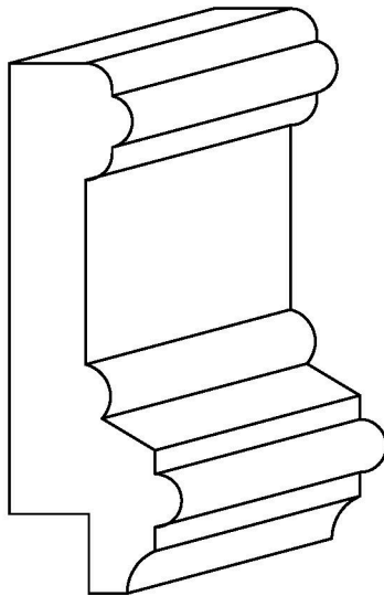
PT 410 Chair Rail 13/16" x 2-1/2" w/ 3/8" or No Rabbet
